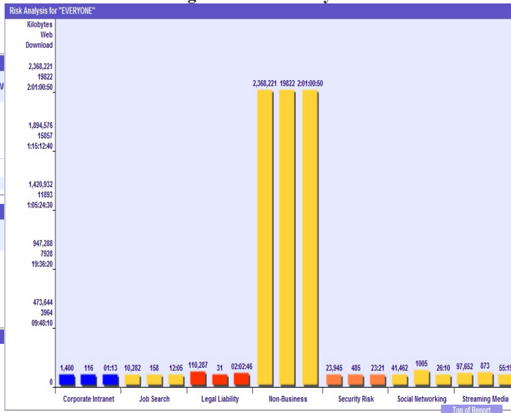
Figure 4: Risk Analysis
