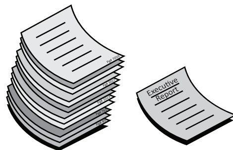
Figure 1: Exception-Based Reporting
